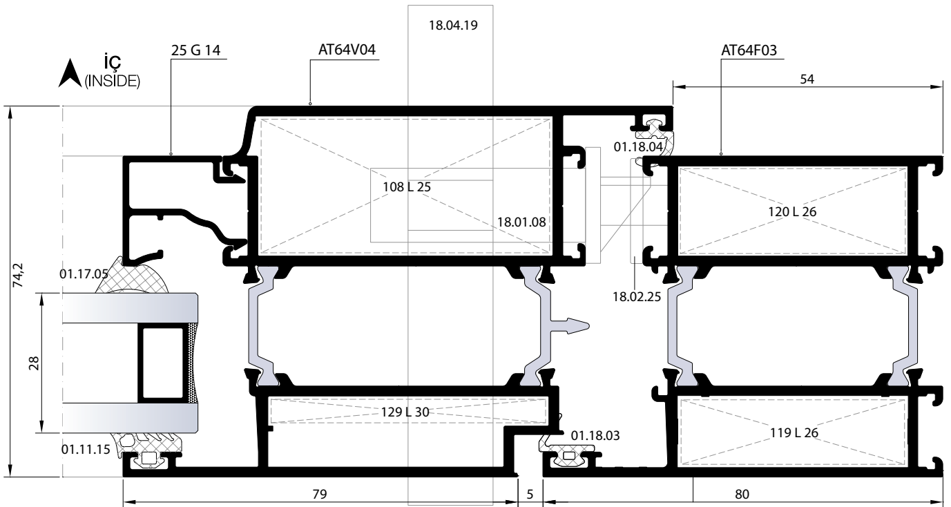
12 DETAYI DETAIL
