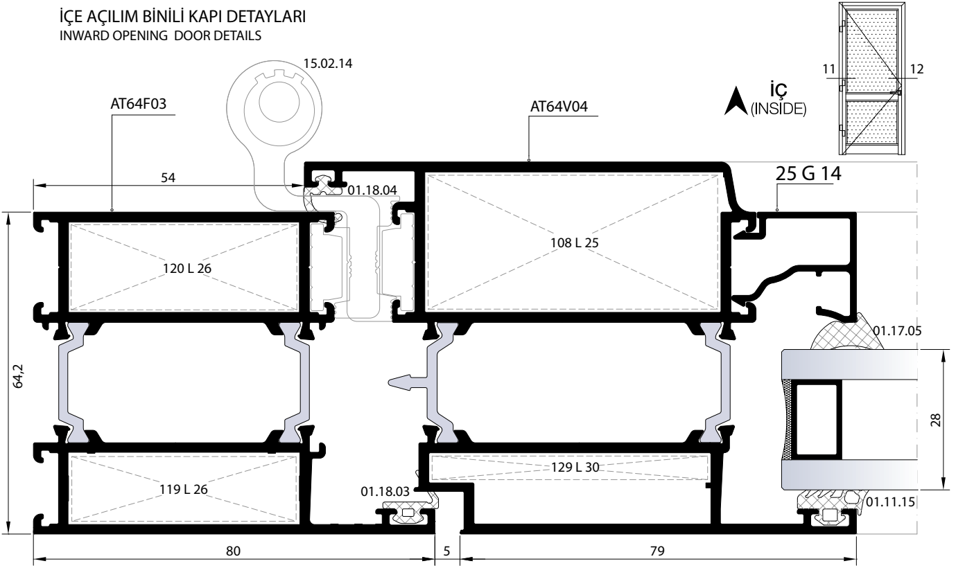
11 DETAYI DETAIL
